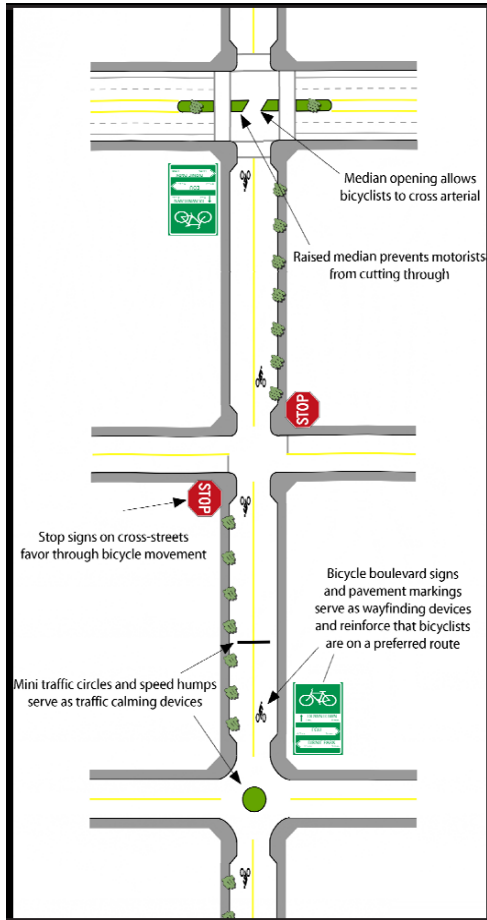
Figure 20: Bicycle Boulevard Diagram
