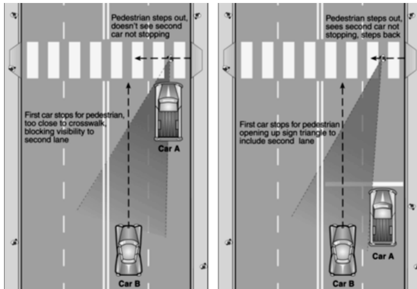
Figure 4: Advance Stop/Yield Bar
